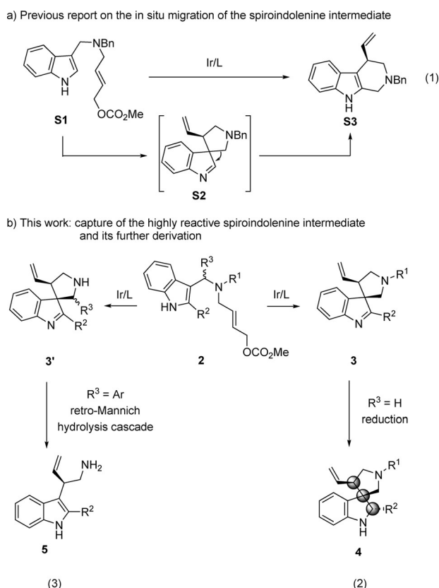
Scheme 1. Derivation of the reactive spiroindolenine intermediates: syntheses of spiroindolines with three contiguous stereogenic centers, and chiral tryptamine derivatives.
